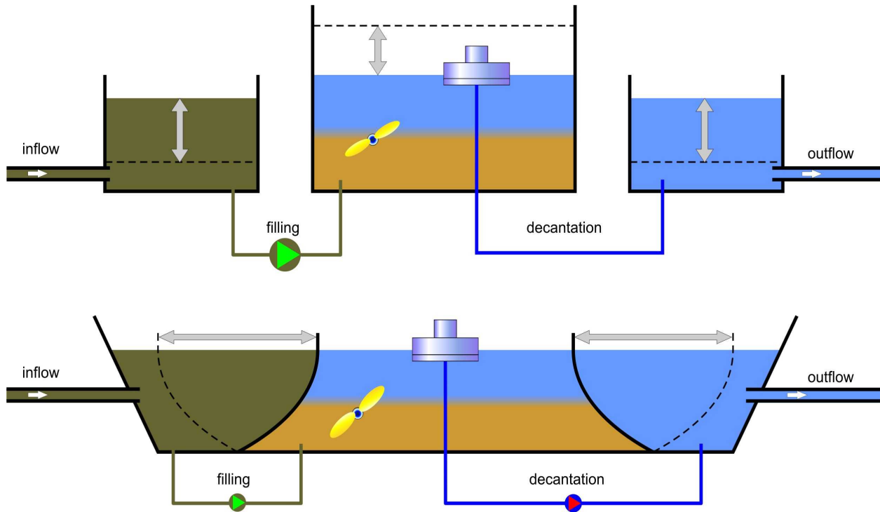
Figure 1: Comparison of water volume changes of CWSBR® and standard SBR.
